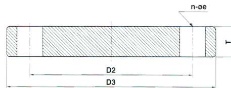
DN15-DN600 BLIND FLANGE
