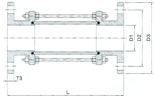
DN15~DN250
